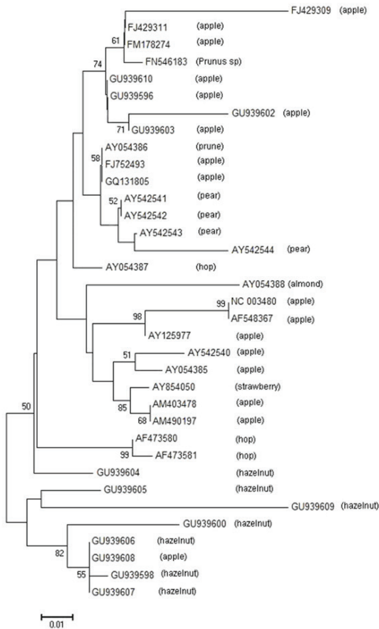
Figure 1. Phylogenetic analysis of nucleotide sequences of coat protein of ApMV isolates. Phylogenetic analysis was obtained using the computer programme of Mega 5 (Tamura et al. 2011). The numbers near nodes were determined by bootstrap analysis (100 replicates)
