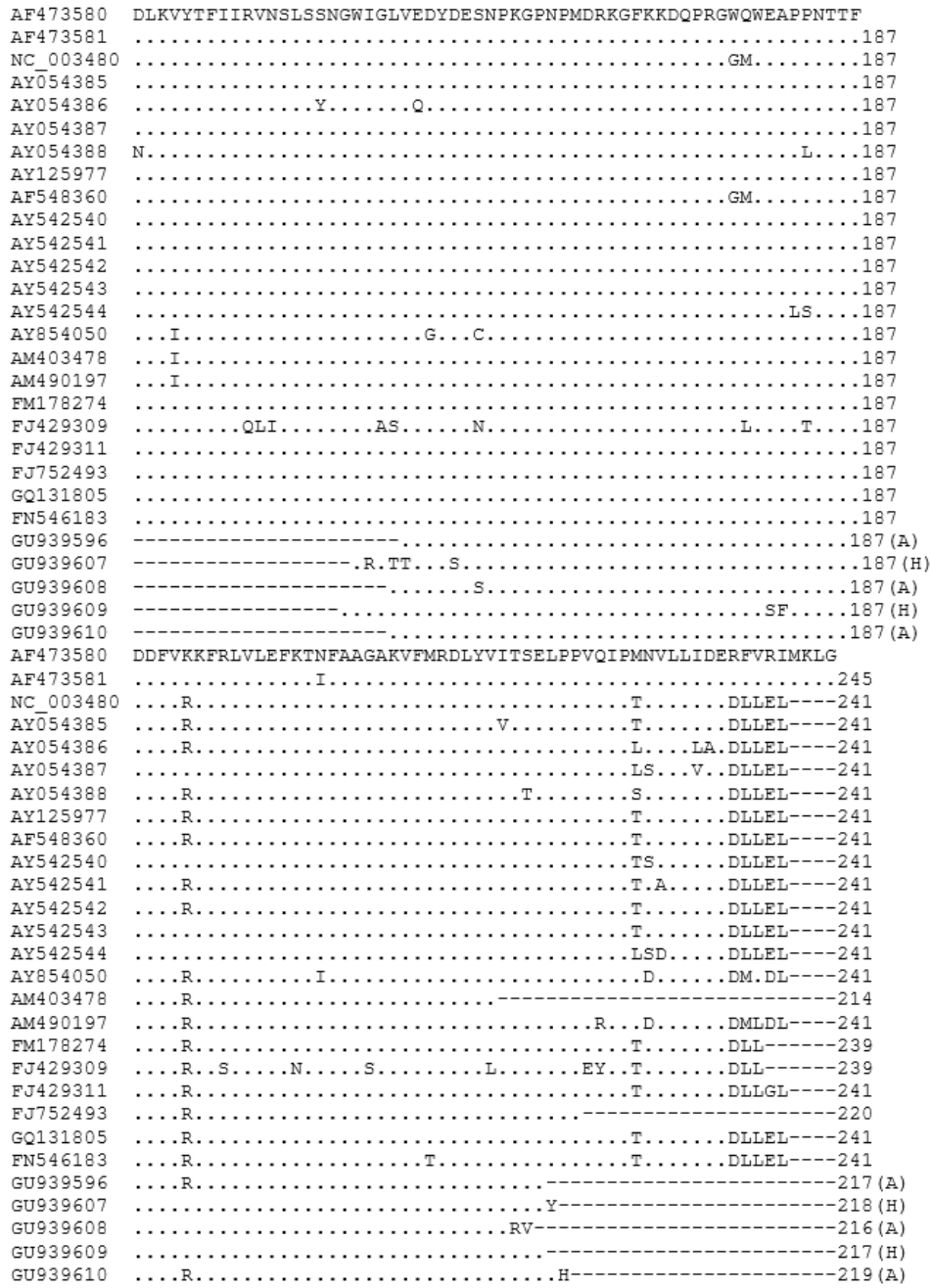
Figure 2. Multiple amino acid sequence alignment of the coat protein of ApMV Turkish isolates deposited in the GeneBank and also those sequences available from GeneBank. Dots indicated identical amino acids and dashes indicates the ends, (A) is apple origin and (H) hazelnut origin. Reference isolate is an coat protein gene of Australian hop strain of ApMV.
