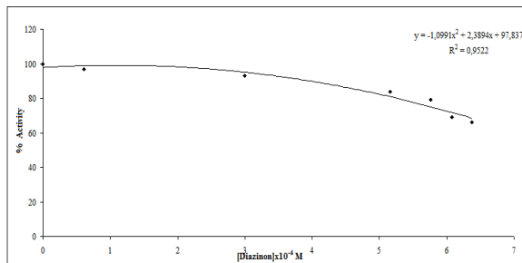
Figure 3. Activity % curve of G6PD in different diazinon concentrations
